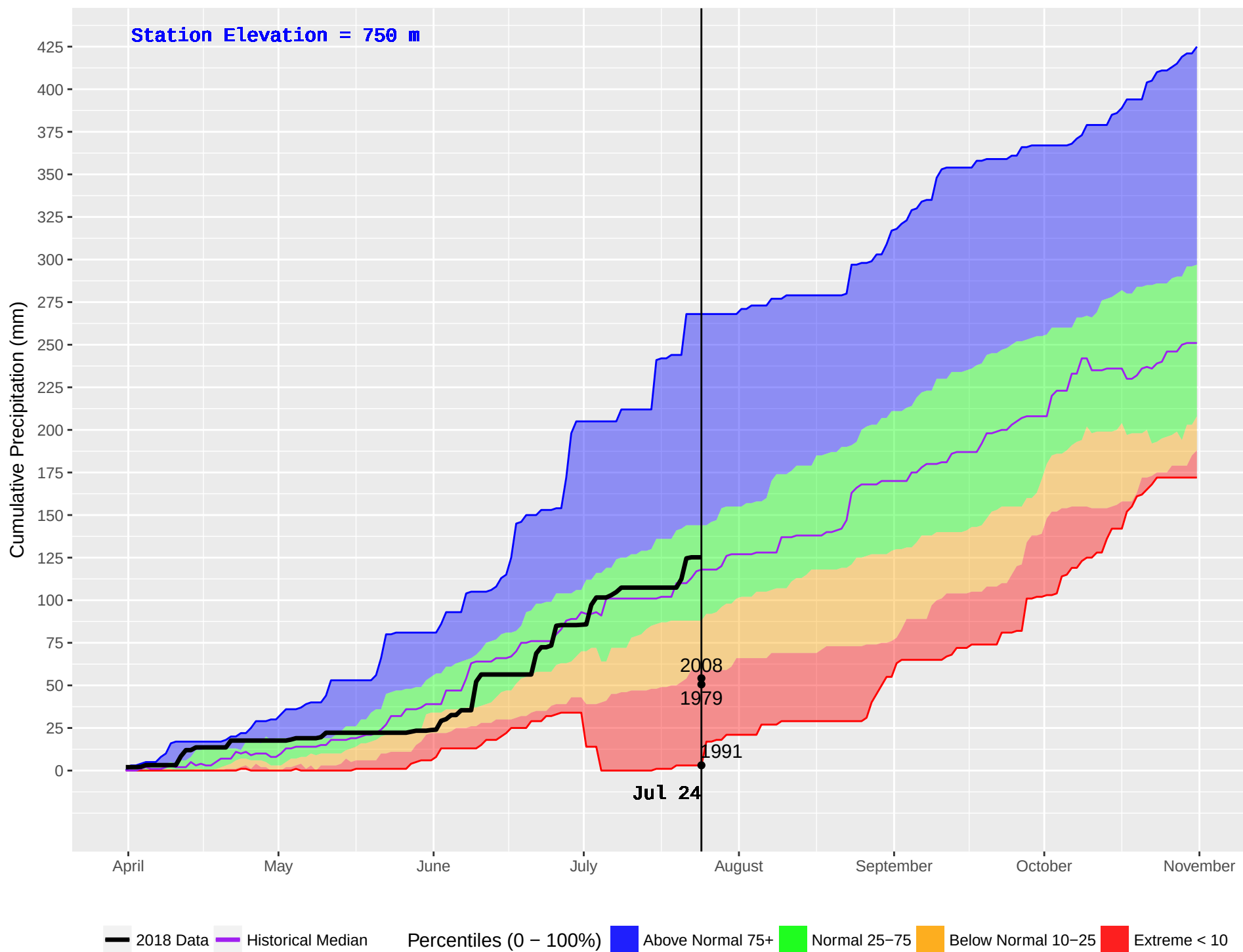
FORT ST JAMES (146) : Historical (1979–2016) and Current (2018) Noon Cumulative Precipitation
