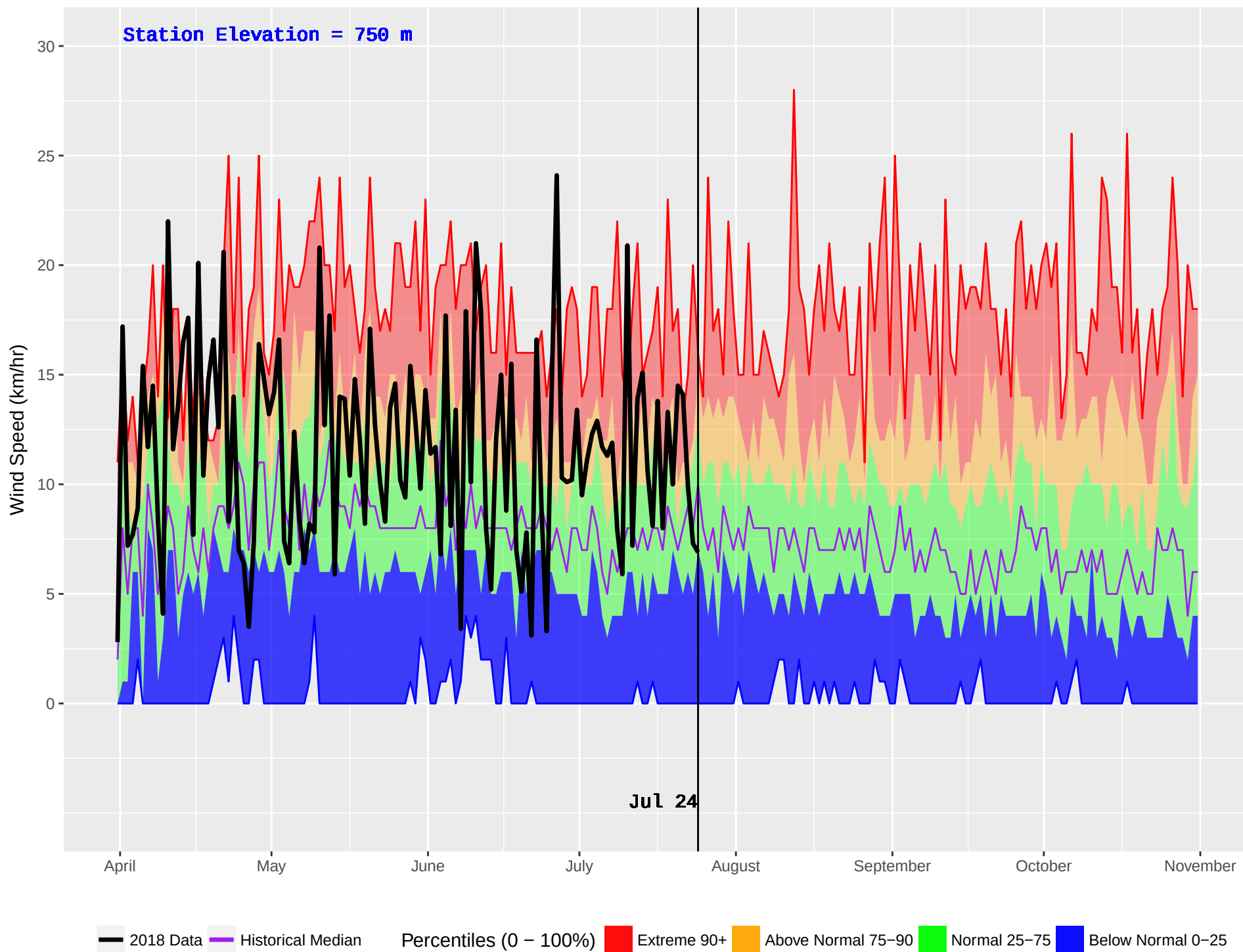
FORT ST JAMES (146) : Historical (1979–2016) and Current (2018) Noon Wind Speed
