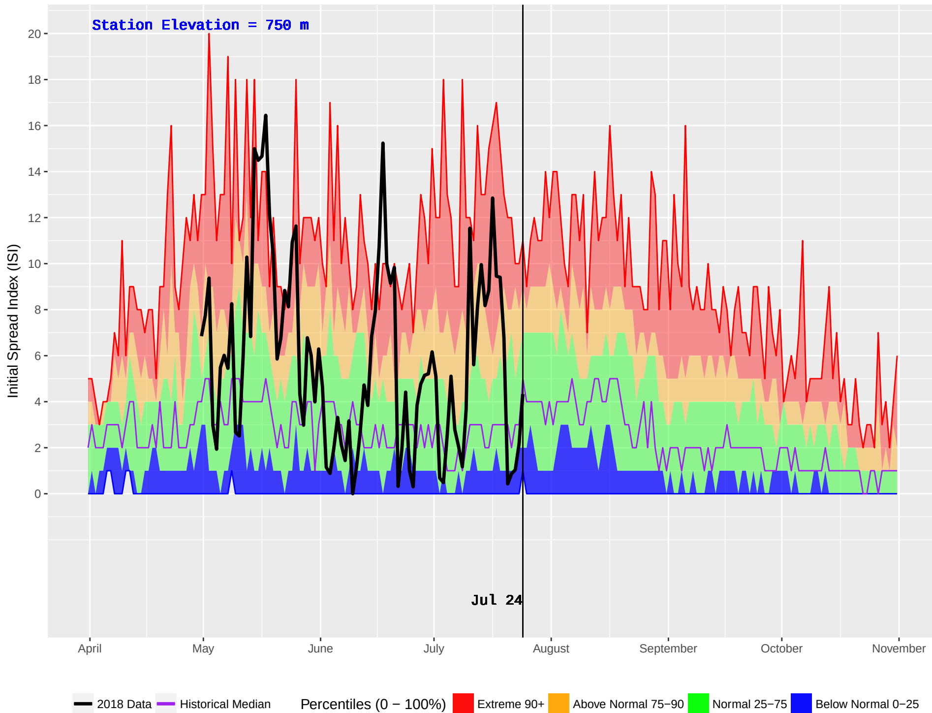
FORT ST JAMES (146) : Historical (1979–2016) and Current (2018) Noon Initial Spread Index (ISI)
