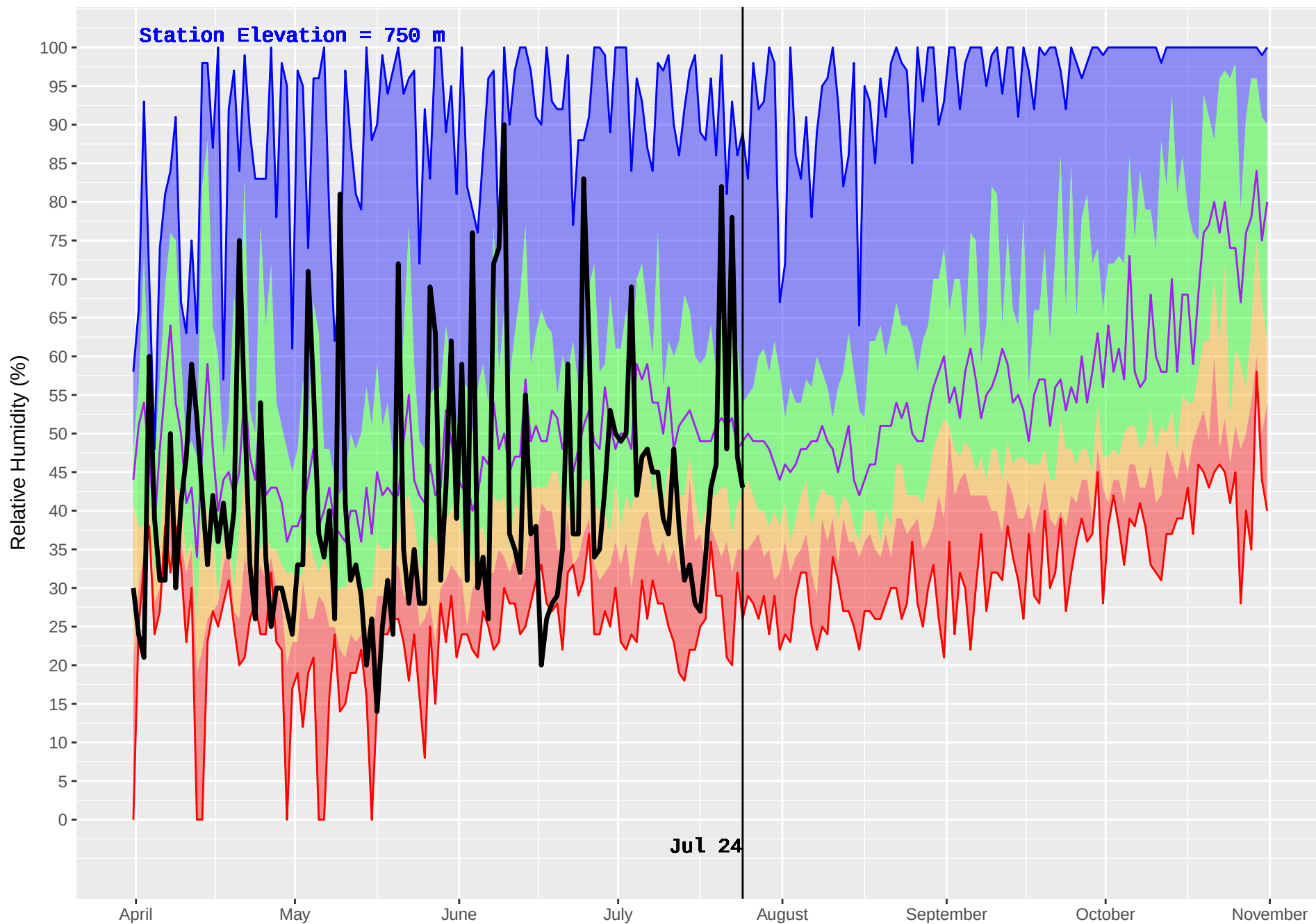
FORT ST JAMES (146) : Historical (1979–2016) and Current (2018) Noon Relative Humidity
