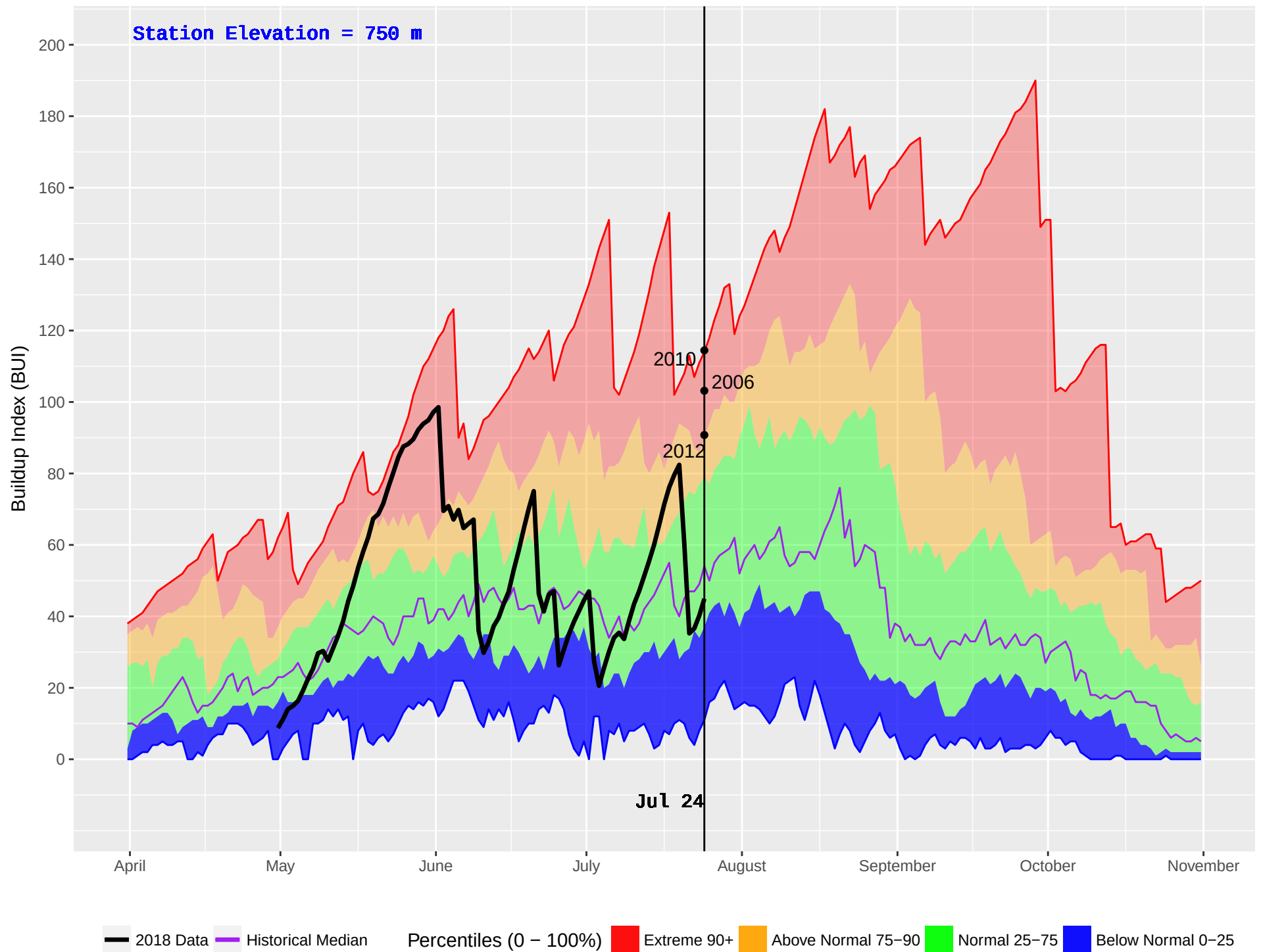
FORT ST JAMES (146) : Historical (1979–2016) and Current (2018) Noon Buildup Index (BUI)
