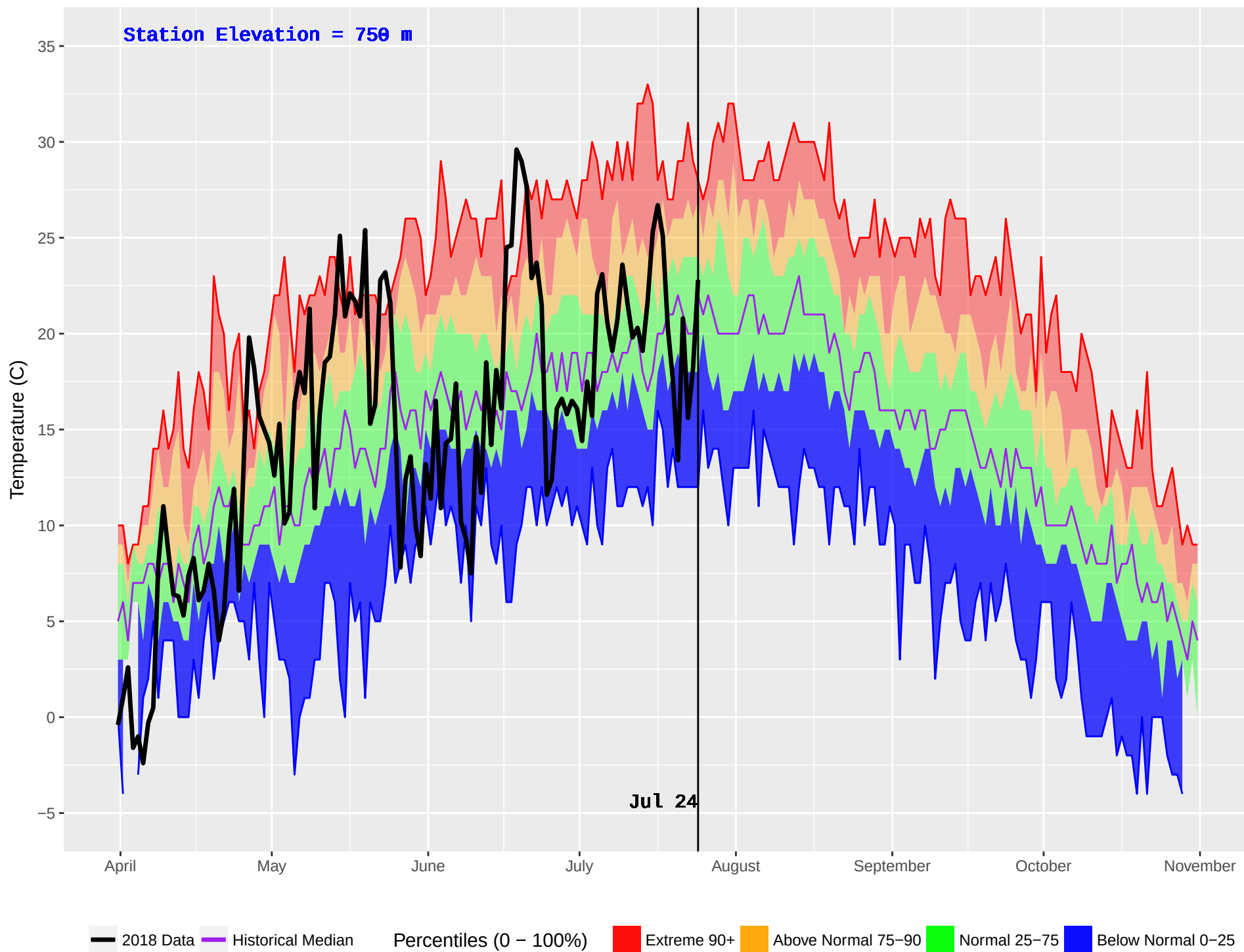
FORT ST JAMES (146) : Historical (1979–2016) and Current (2018) Noon Temperature
