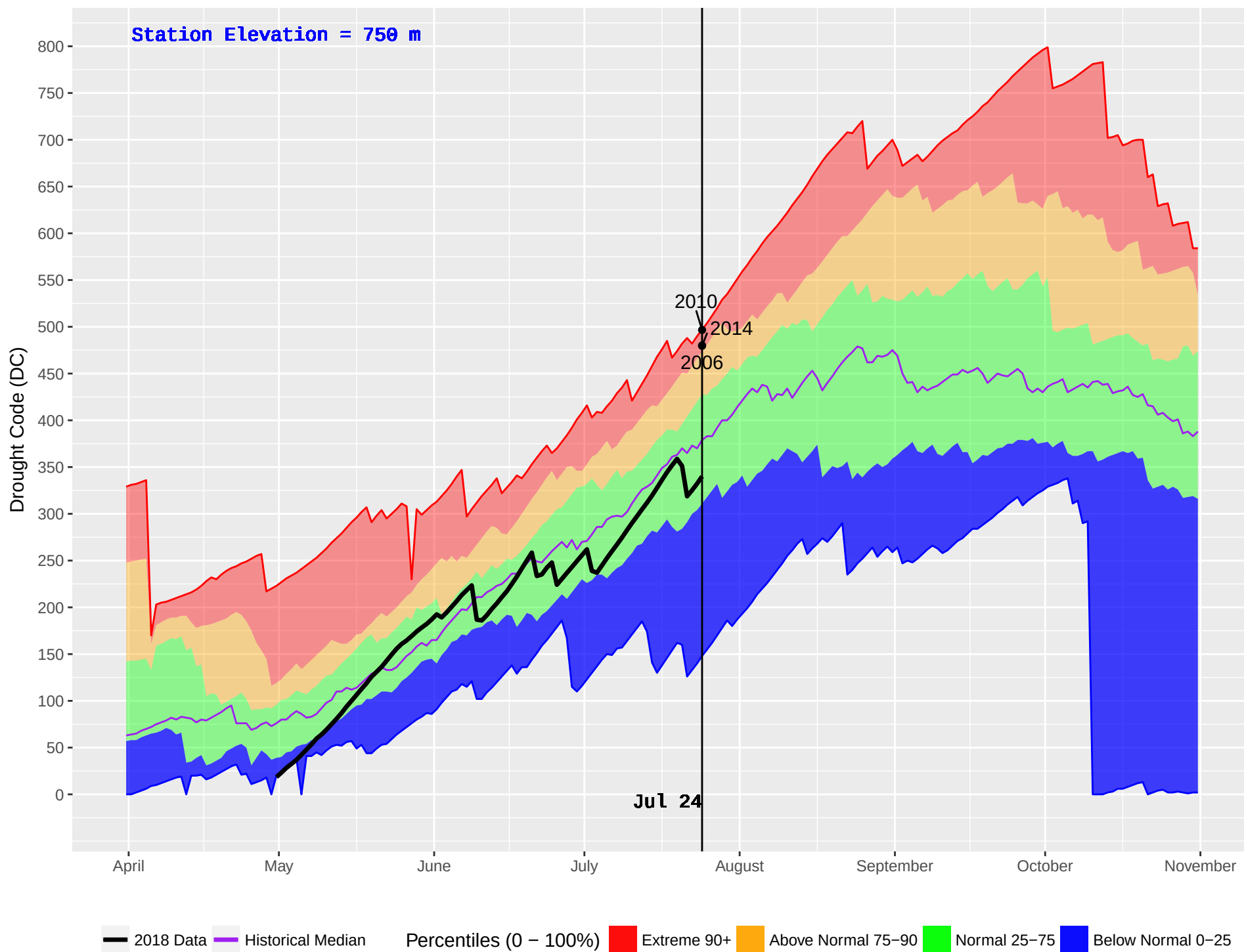
FORT ST JAMES (146) : Historical (1979–2016) and Current (2018) Noon Drought Code (DC)
